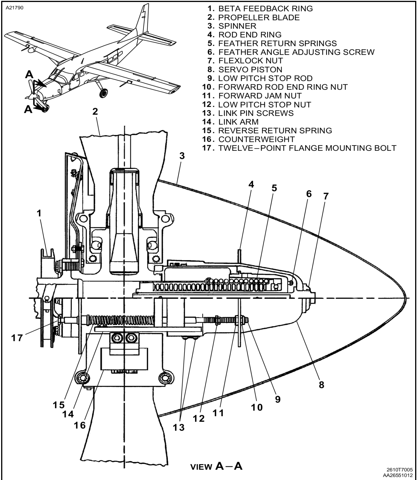
Figure 1 : Sheet 1 : Hartzell Propeller Assembly Cutaway
